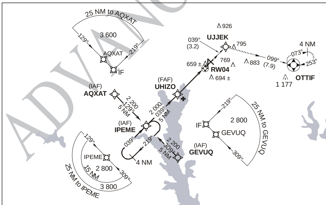
Figure I-2-3-5. "T" bar icon arrangement without centre initial approach fix
