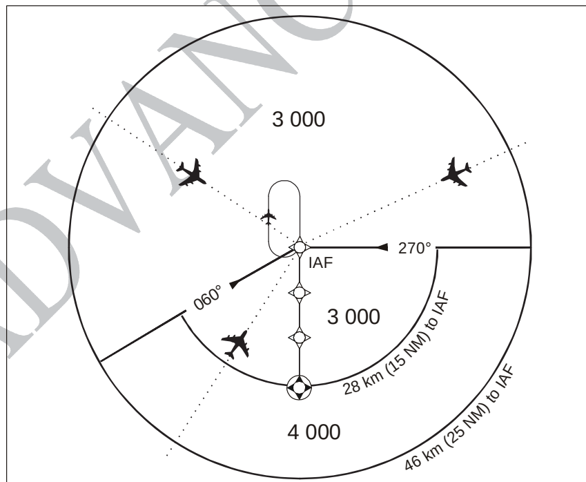
Figure II-1-2-9. Single TAA with sectorization and stepdown
