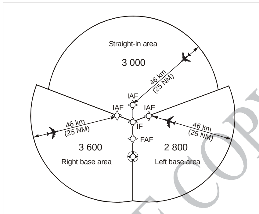
Figure II-1-2-1. Typical TAA arrangement
