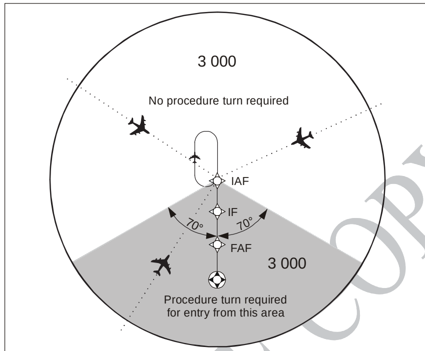
Figure II-1-2-8. TAA arrangement without left and right base
