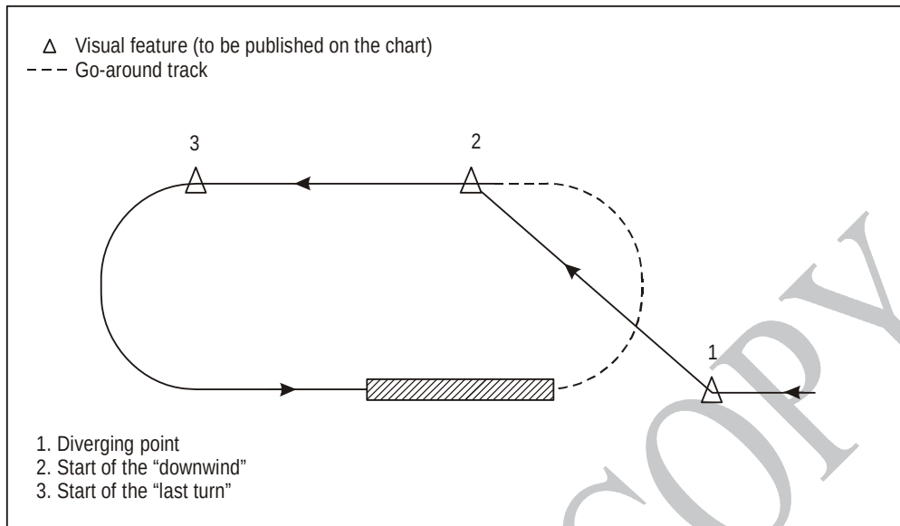
Figure I-4-7-3. Standard track general case
