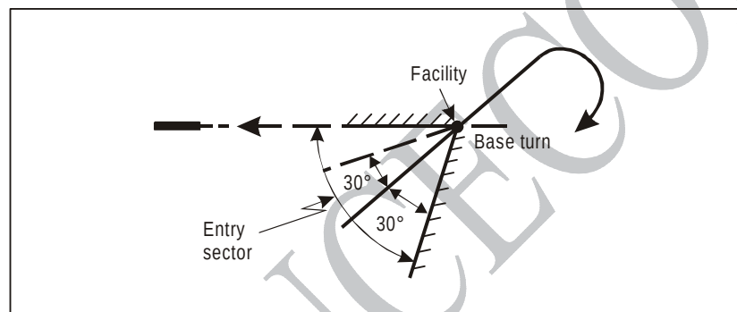
Figure I-4-3-3. Direct entry to base turn
