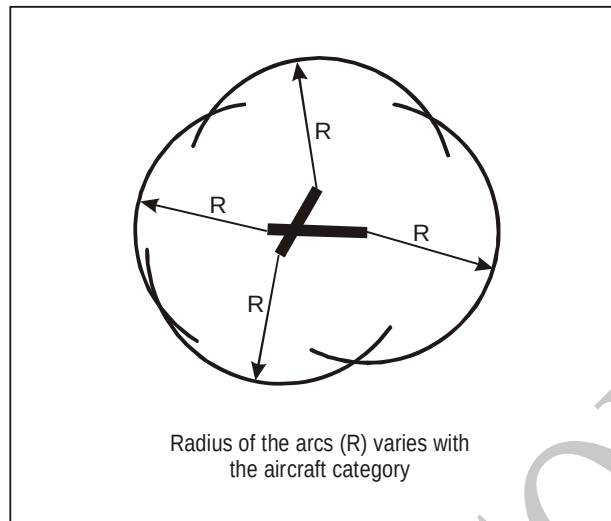
Figure I-4-7-1. Visual manoeuvring (circling approach) area
