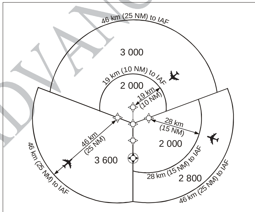
Figure II-1-2-2. TAA with stepdown arcs
