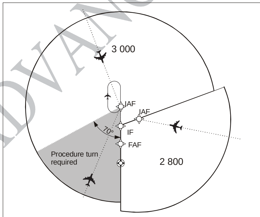
Figure II-1-2-7. TAA arrangement without right base
